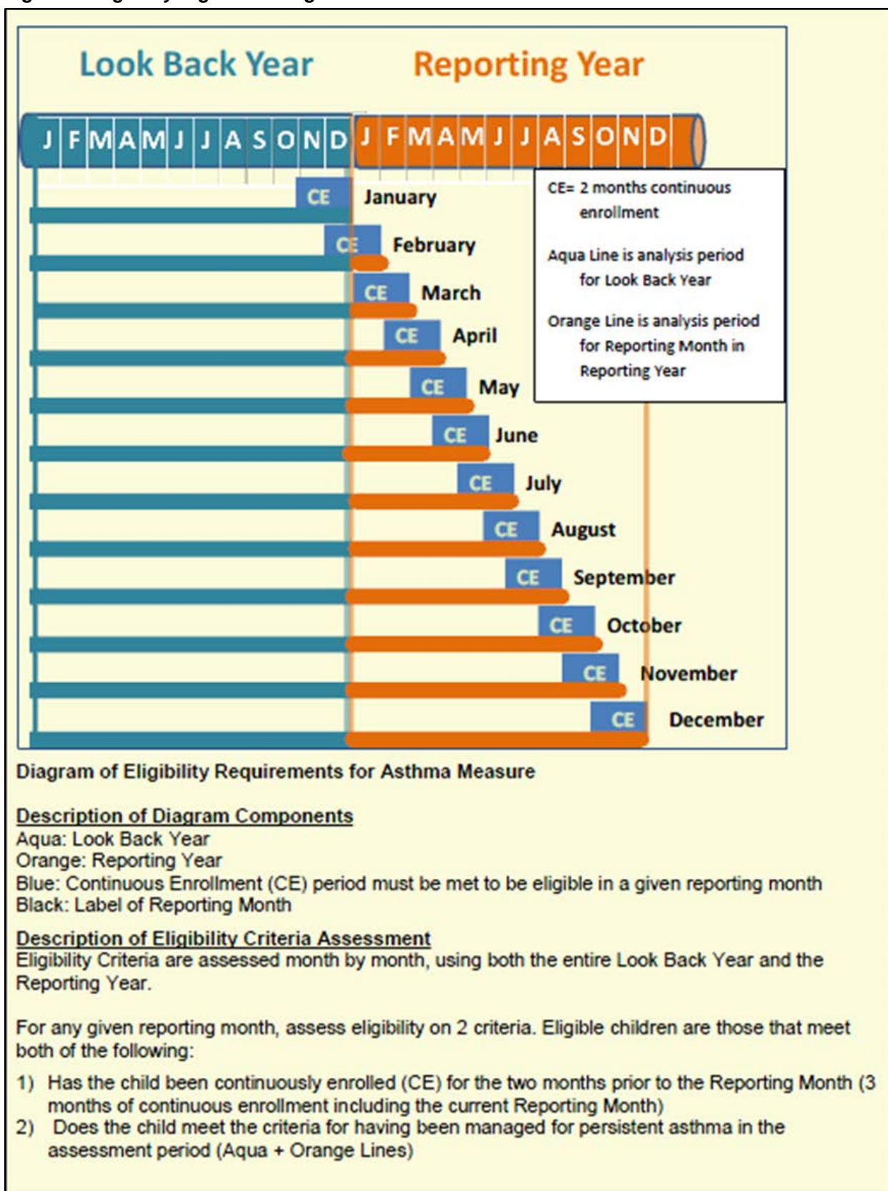
Figure 1. Eligibility Algorithm Diagram
